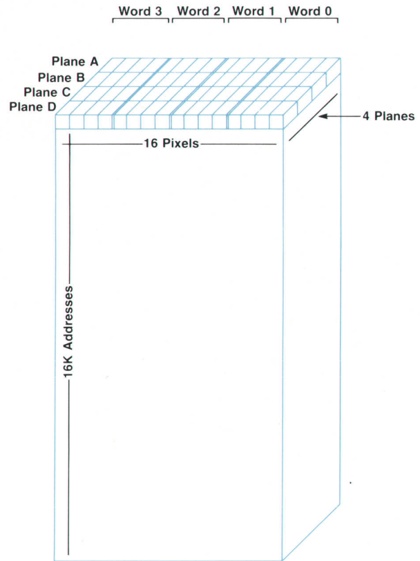
Fig. 4. Logical organization of the image memory array.
