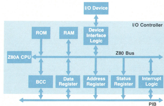
Fig. 2. An I/O channel on the processor-independent bus (PIB).
